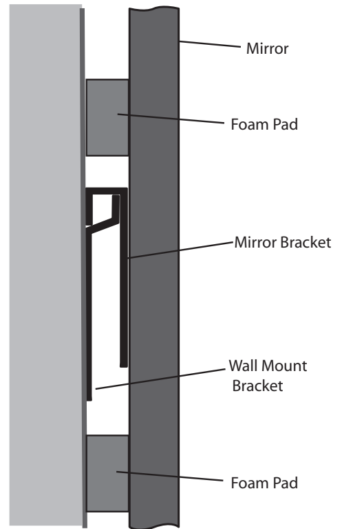
mounted mirror section view
