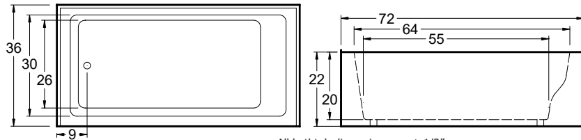
All bathtub dimensions are ± 1/2".
