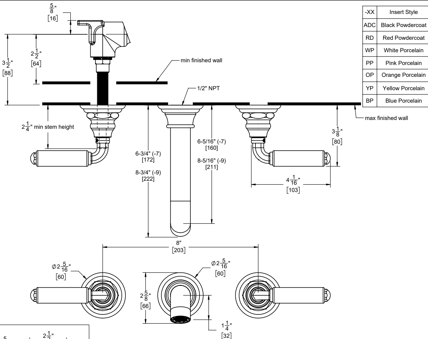
TO-V6002-7-SN shown
