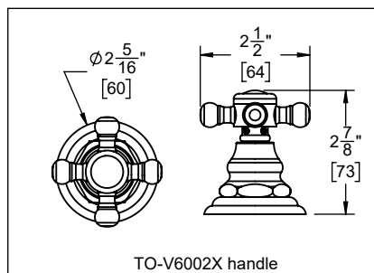
TO-V6002X handle
