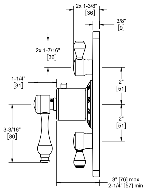
TO-THC2L-61 side view
