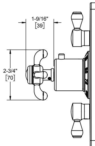
TO-THC2L-61XD side view
