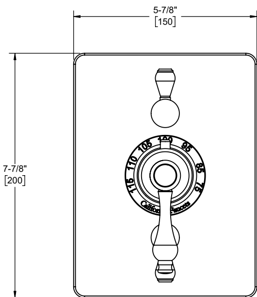
TO-THC2L-61 front view
