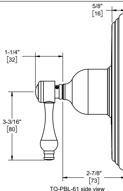
TO-PBL-61 side view
