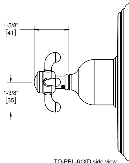
TO-PBL-61XD side view
