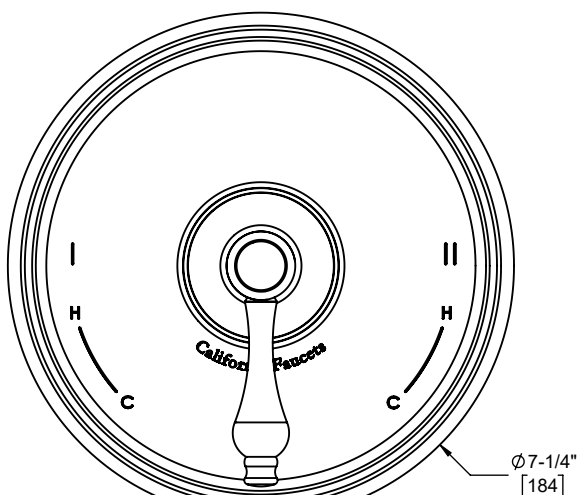
TO-PB2L-61 front view
