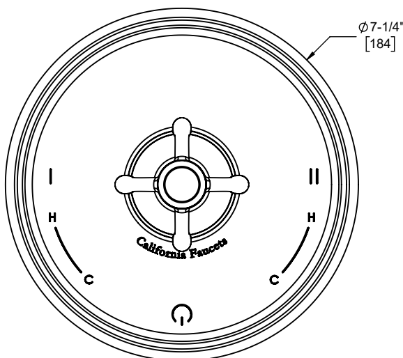
TO-PB2L-61XD front view
