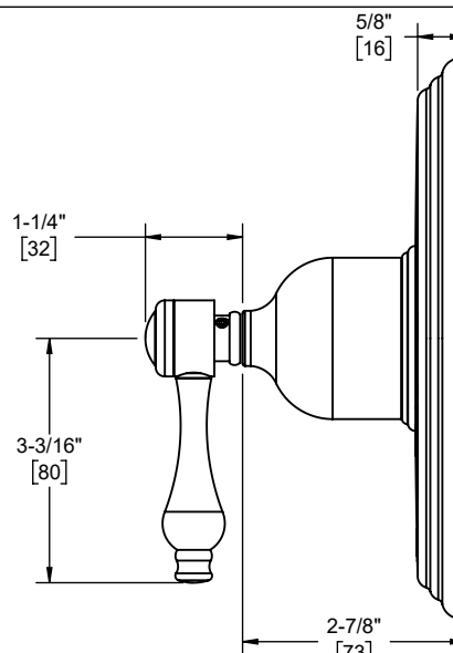
TO-PB2L-61 side view
