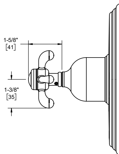
TO-PB2L-61XD side view
