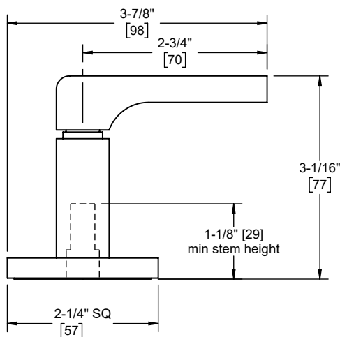
TO-70-W shown
