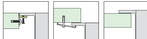
Flush-mount
