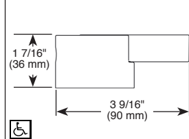
HL7032▲ Lever Handle
