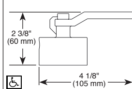
HL7034▲ Industrial Lever Handle
