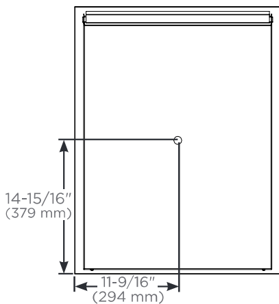
Back view for electrical knockout location
