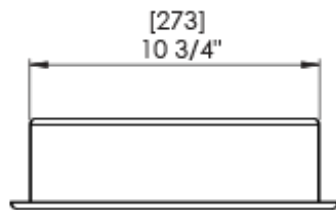
12" X 24" RECESSED WALL NICHE WITH TWO ADJUSTABLE SHELVES (FOR VERTICAL USE)
