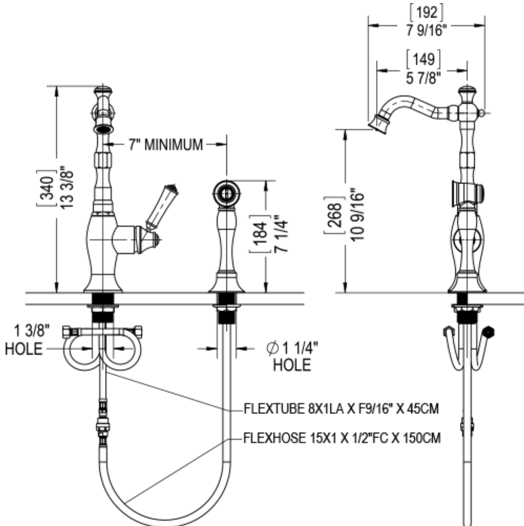
SINGLE CONTROL BAR FAUCET WITH HAND SPRAY
