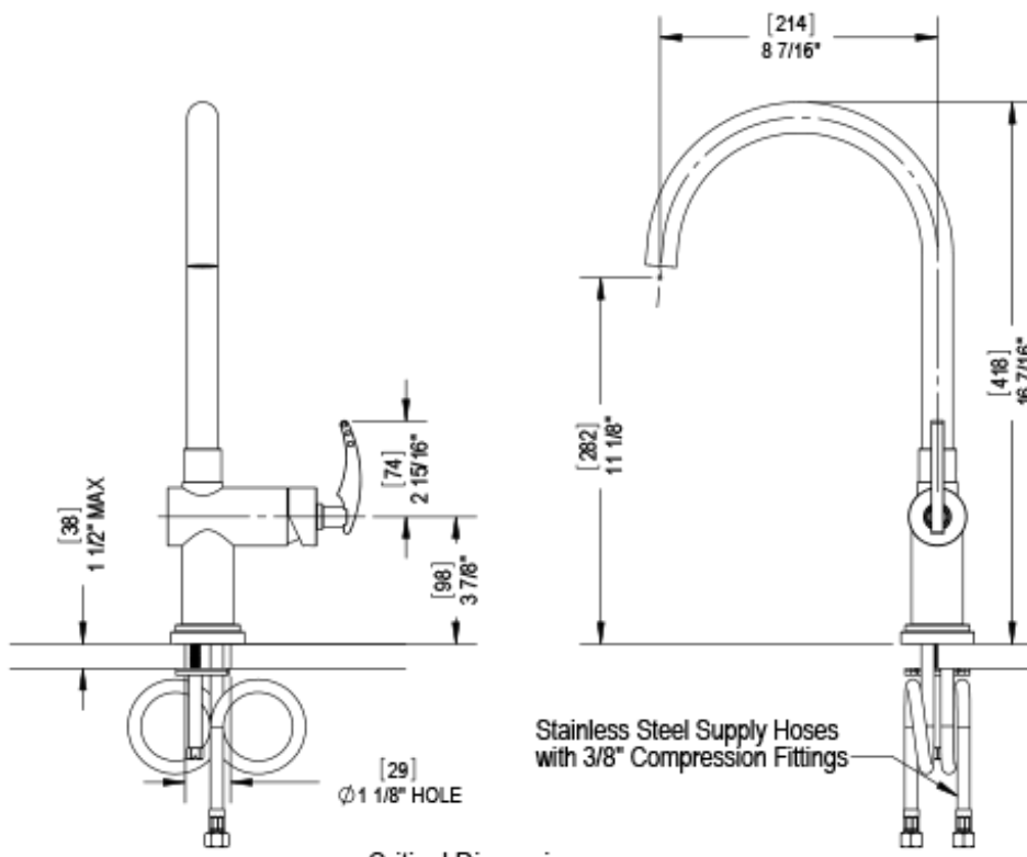
Critical Dimensions
