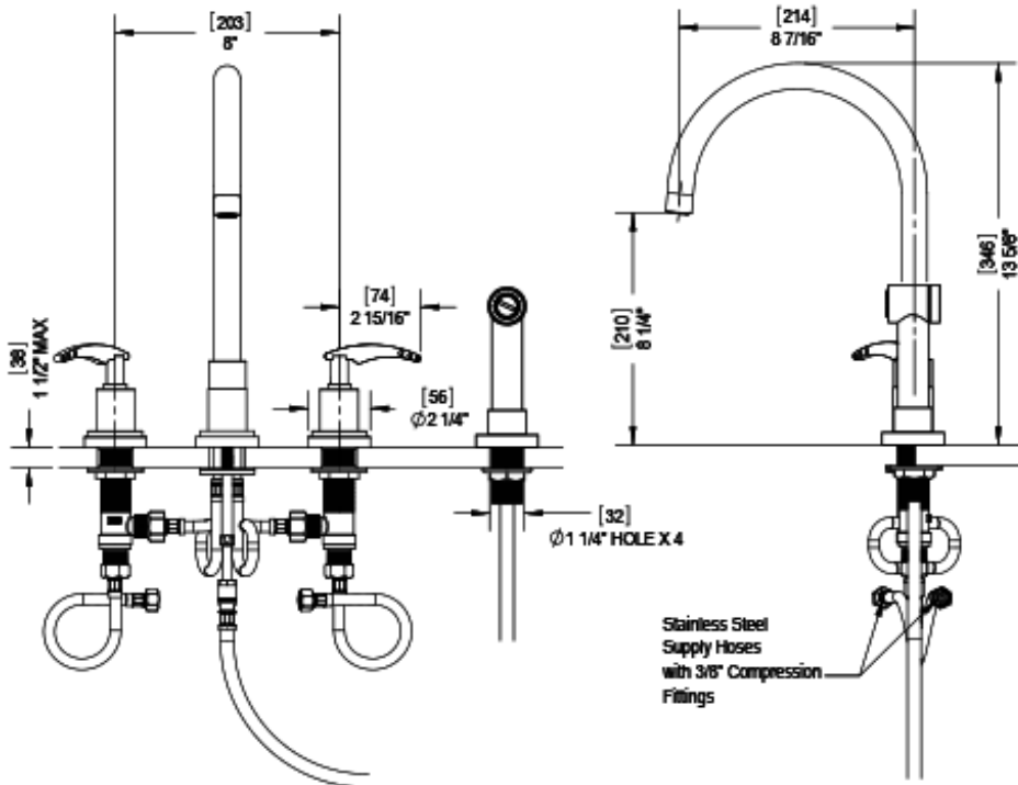
Critical Dimensions
