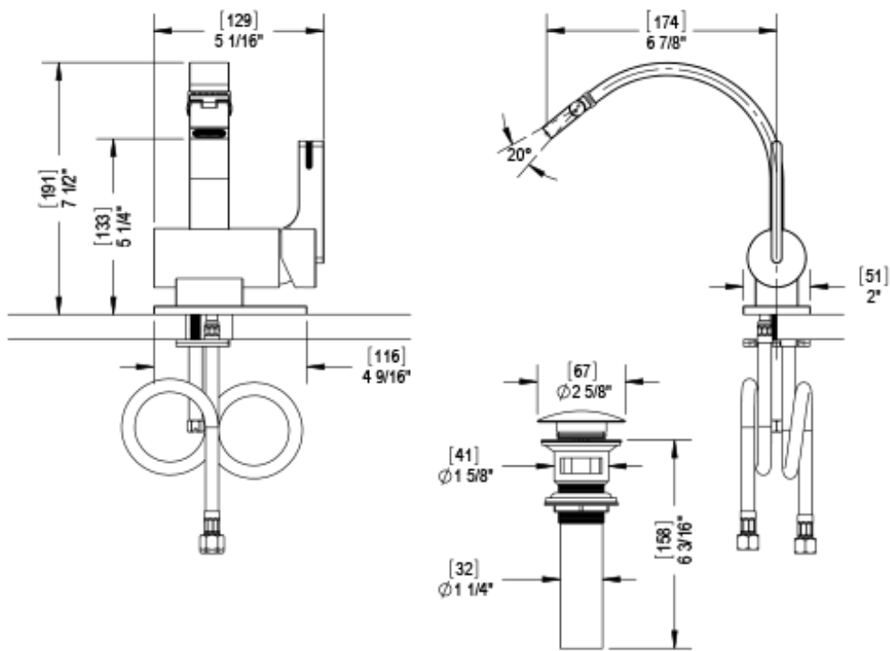
Critical Dimensions
