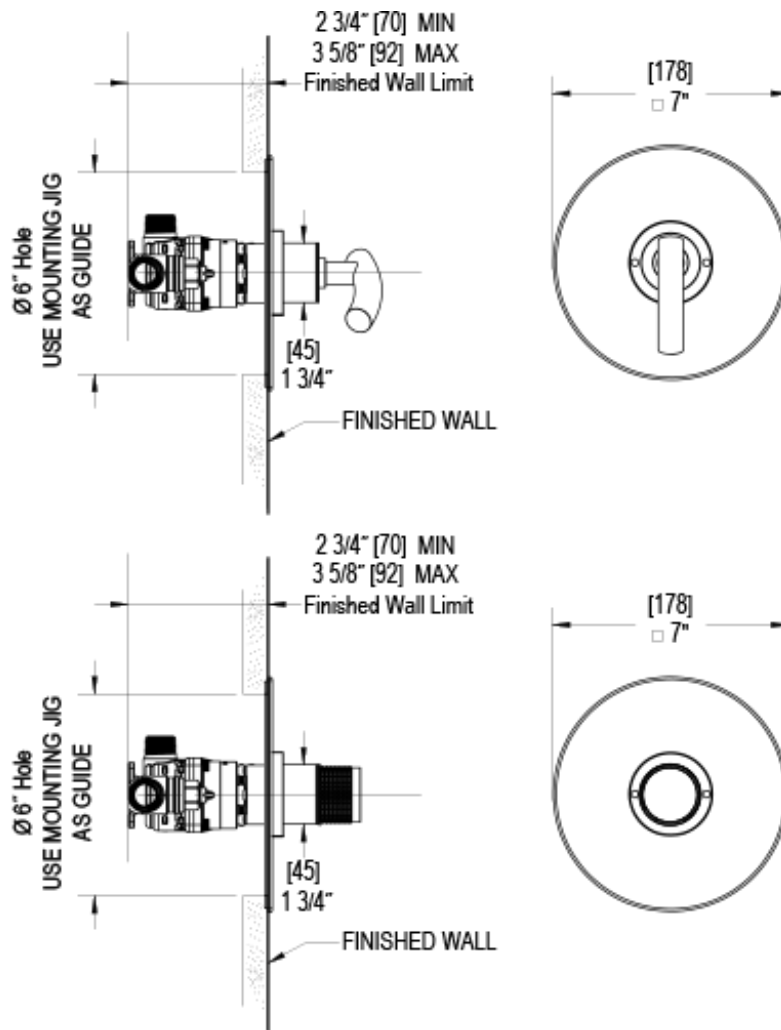
PRESSURE BALANCE SHOWER VALVE WITH STOPS
