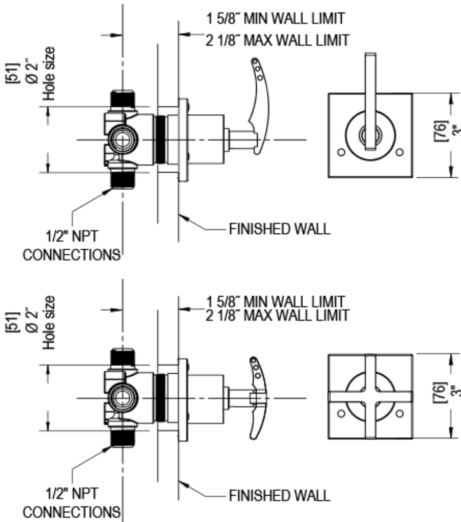
THREE WAY DIVERTER VALVE WITH SHARED OUTLETS IN BETWEEN FUNCTIONS
