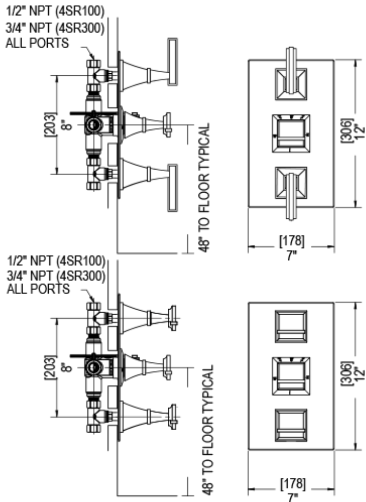
TEMPERATURE CONTROL VALVE WITH STOPS & TWO VOLUME CONTROLS
