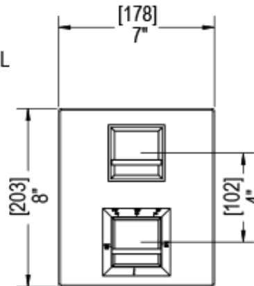
TEMPERATURE CONTROL VALVE WITH STOPS & VOLUME CONTROL
