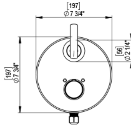
TEMPERATURE CONTROL VALVE WITH STOPS & VOLUME CONTROL
