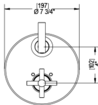
TEMPERATURE CONTROL VALVE WITH STOPS & VOLUME CONTROL
