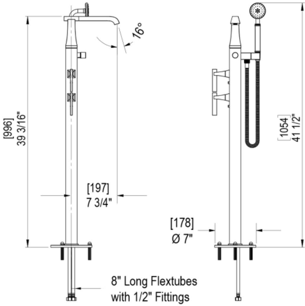
FLOOR MOUNT TUB FILLER WITH HAND HELD SHOWER
