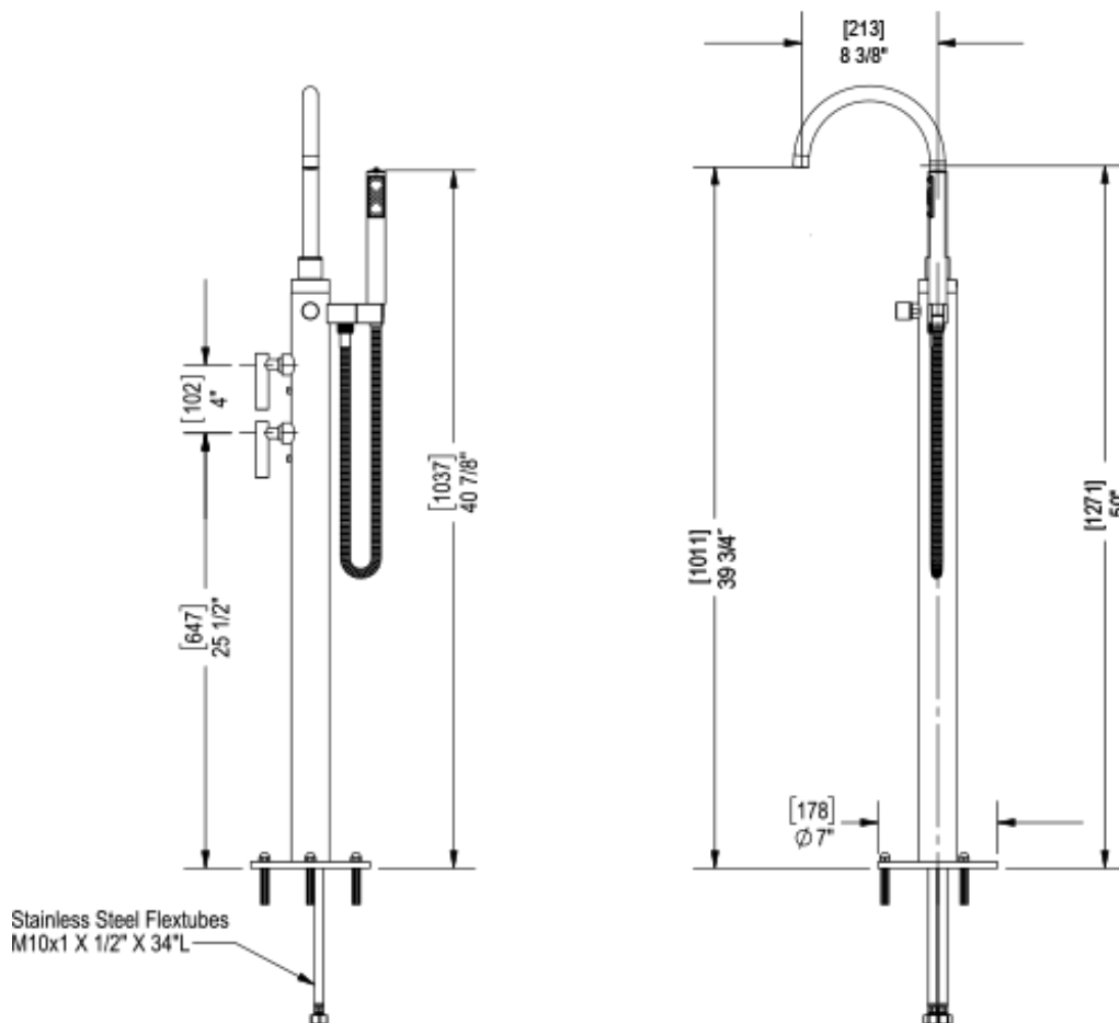
FLOOR MOUNT TUB FILLER WITH HAND HELD SHOWER, LASALLE SPOUT
