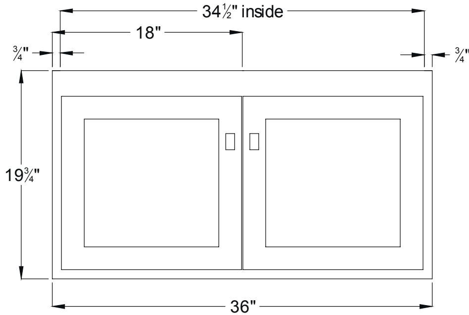
Front View
