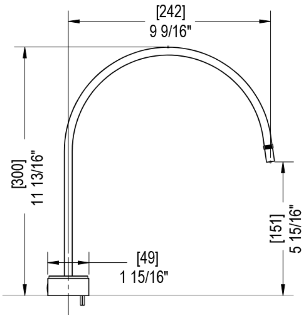
DECK MOUNT TUB SPOUT
