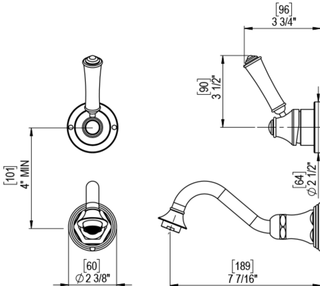
WALL MOUNT SINGLE CONTROL LAV (LESS DRAIN)
