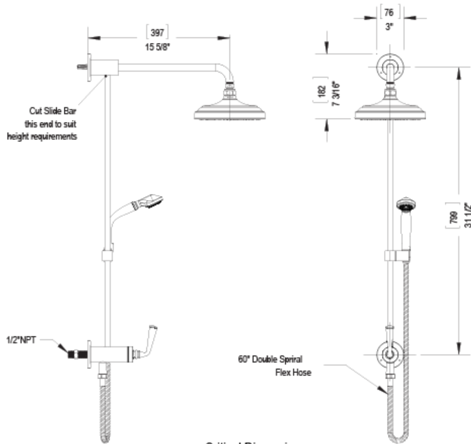
Critical Dimensions
