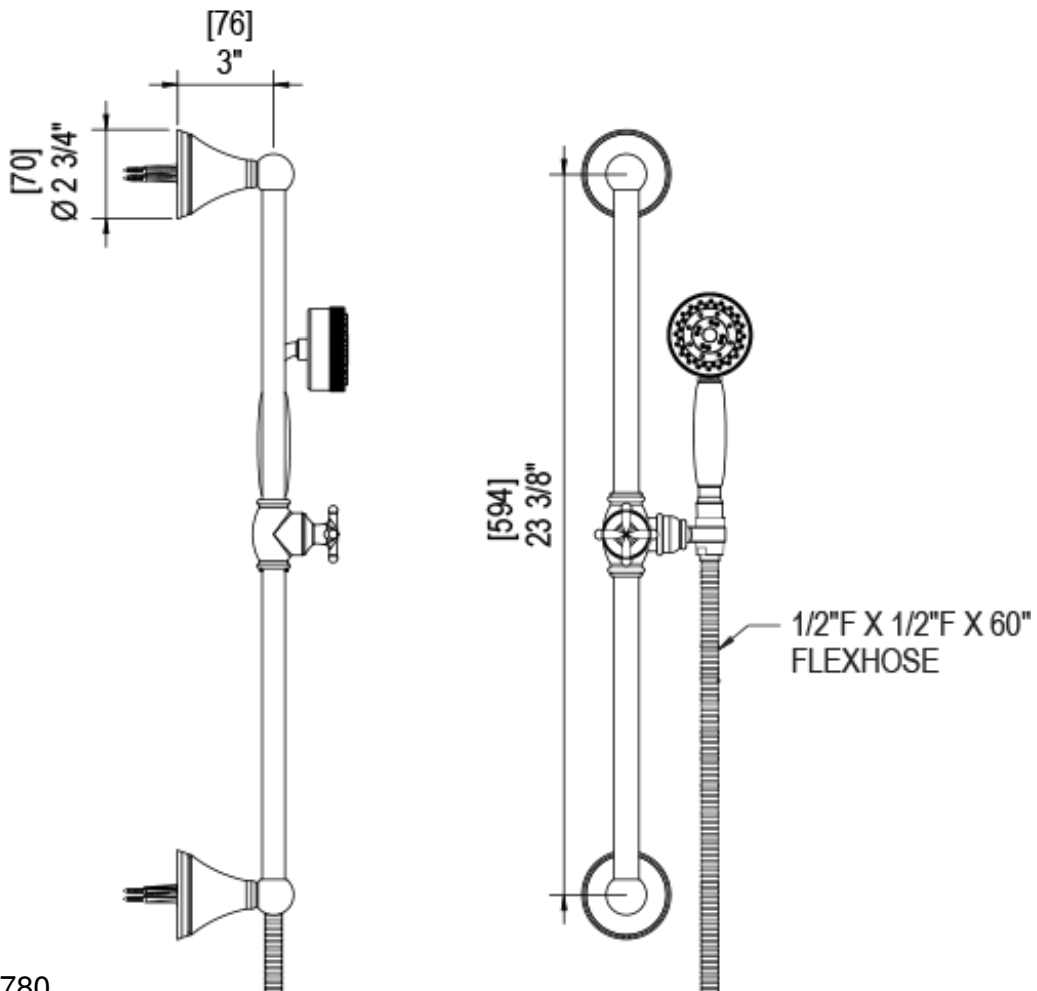
ADJUSTABLE SLIDE BAR WITH HAND HELD SHOWER ASSEMBLY 3 FUNCTION
