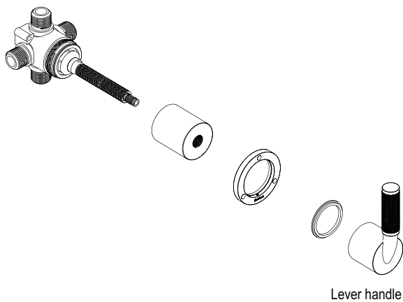
4XR100 Rough-In Valve
