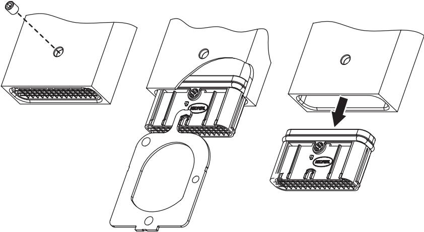
DISASSEMBLING KEY
