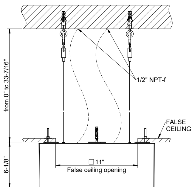
INSTALLATION MODE 1
