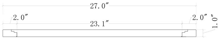
TOP VIEW
