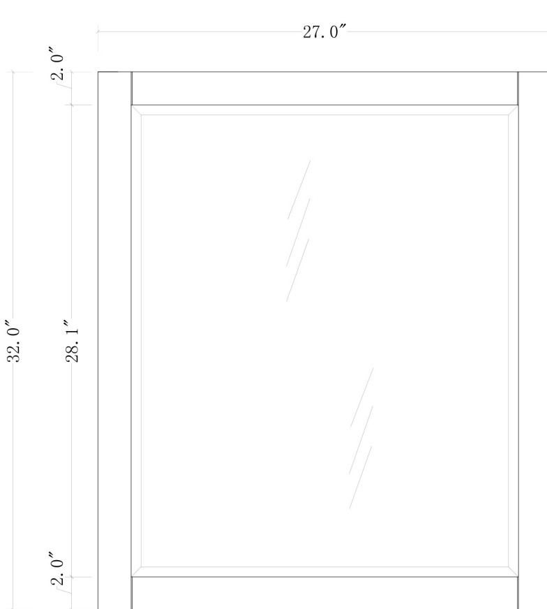
FRONT VIEW
