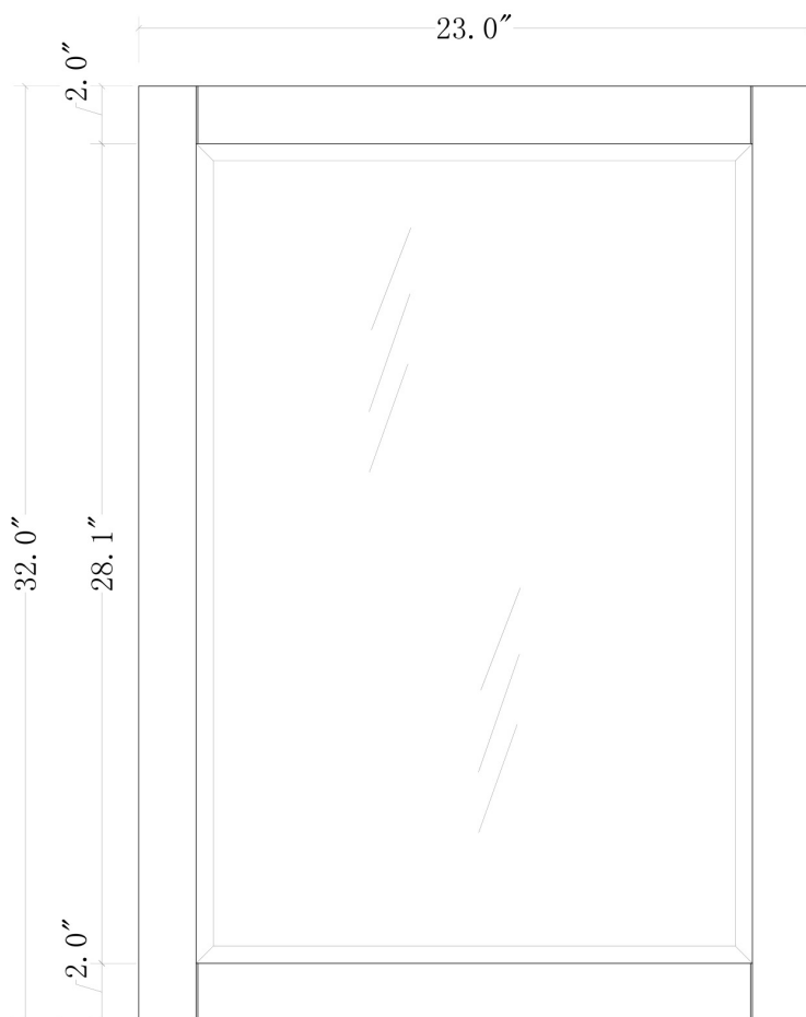
FRONT VIEW
