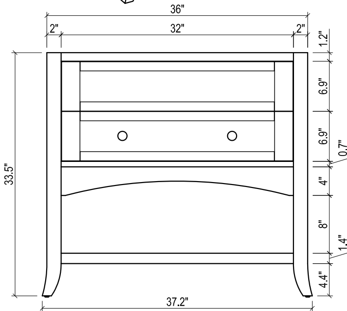
FRONT VIEW
