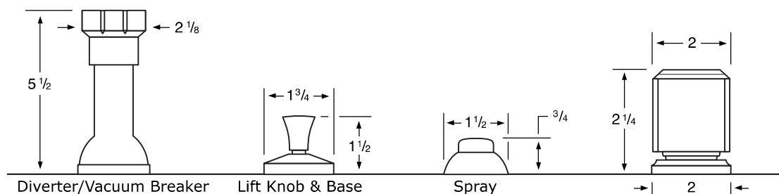
Diverter/Vacuum Breaker
