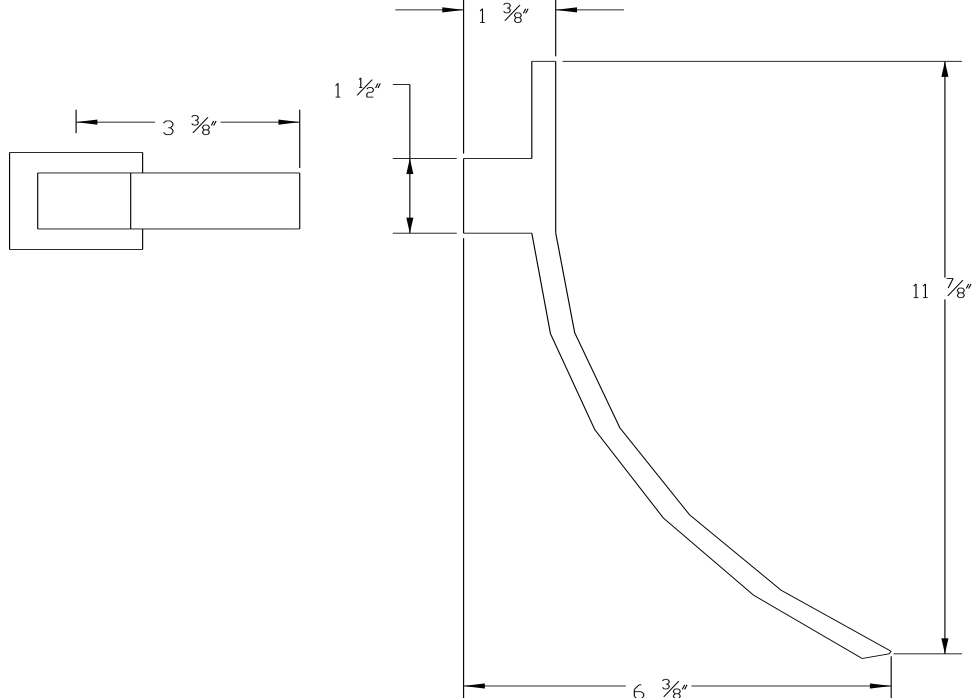
SIDE VIEW
