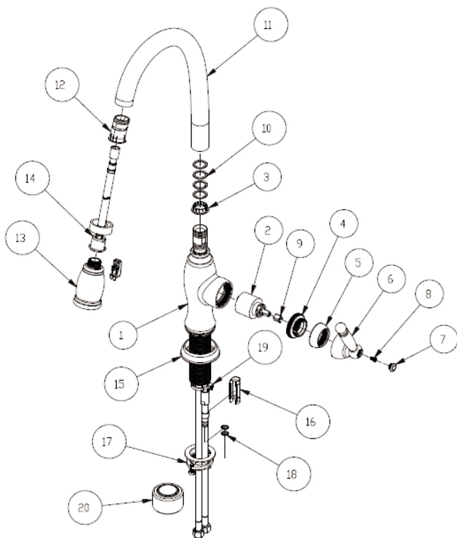
Figure 6 - Spare Parts
