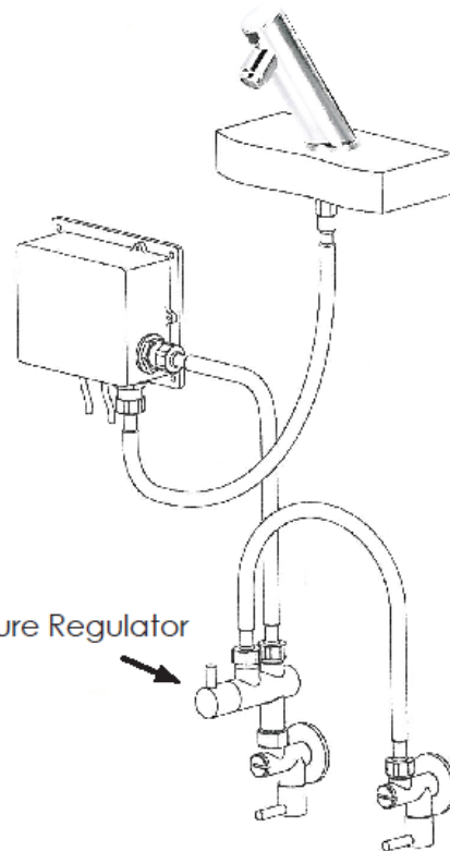
2 Inlet Sensor Faucet with Temperature Regulator
