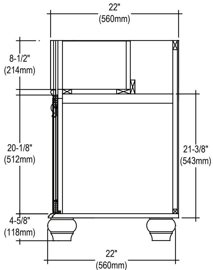
4. Side view line drawing
