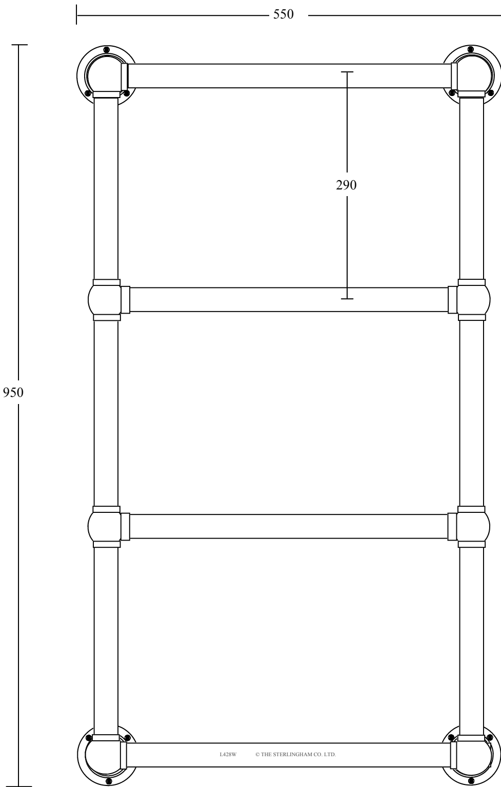
MODEL L428W Overall size 950 high x 550 wide
