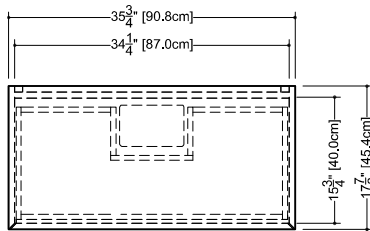
plan view
