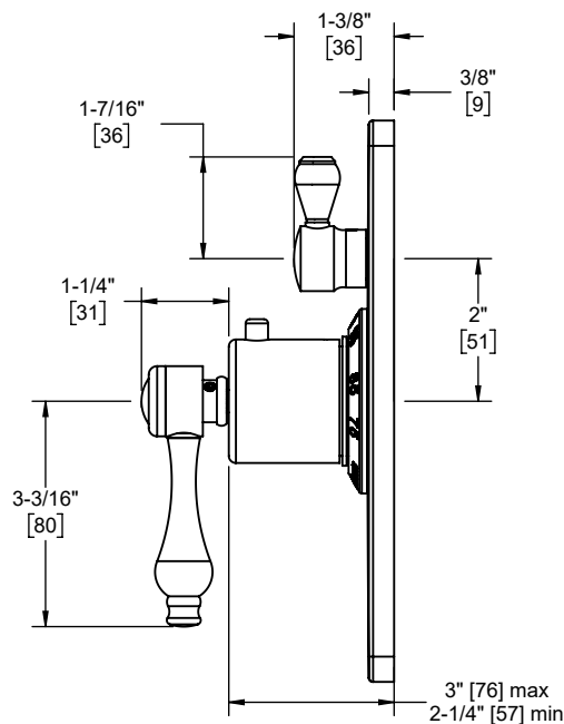
TO-THC1L-61 side view
