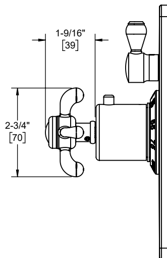
TO-THC1L-61XD side view
