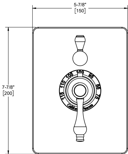
TO-THC1L-61 front view
