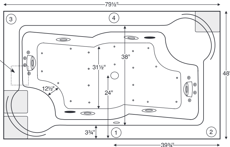
Numbered areas on tub deck represent possible locations to install cleaning systems, faucets and other fixtures. Shown with Air Massage and Ultra Whirlpool Package.
