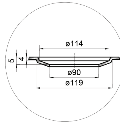
Detail 1 – Drain (1:2.5)
