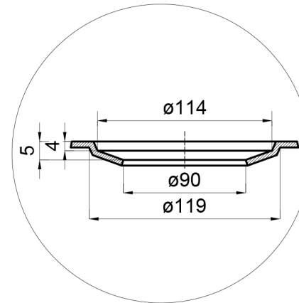
Detail 1 – Drain (1:2.5)
