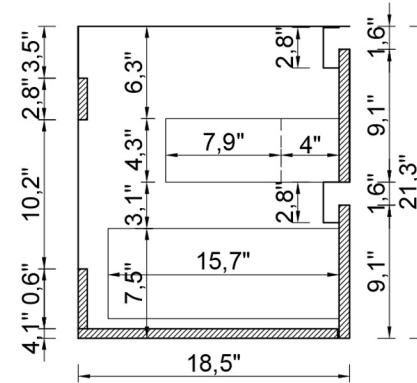
CROSS VIEW
